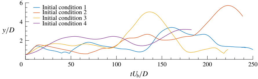
FIGURE 4. Time history of the bed-normal position of the centre of the sediment particle for the different realisations considered at Ga_{25} , all with incipient motion.
