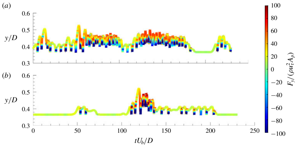
FIGURE 12. Time history of the normal position of the moving particle for (a) Ga250 and (b) Ga310 , coloured by the normal force, F_y , exerted on the particle by the fluid, scaled with (\rho u_t^2 A_p) .
