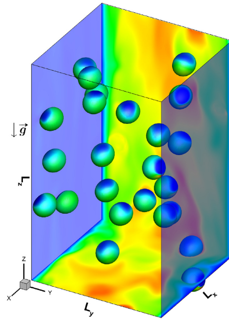
Fig. 1. Schematic representation of the computational setup considered in the present work. The contours on the plane represent streamwise velocity with the scale ranging from 0.15W_b^* (blue) to 1.1W_b^* (red) where W_b^* is the average bulk velocity in the single-phase case. The contours on the bubble surface represent interfacial surfactant concentration ( \Gamma ) with the scale ranging from 0 (blue) to 0.15 (red). (For interpretation of the references to colour in this figure legend, the reader is referred to the web version of this article.)
